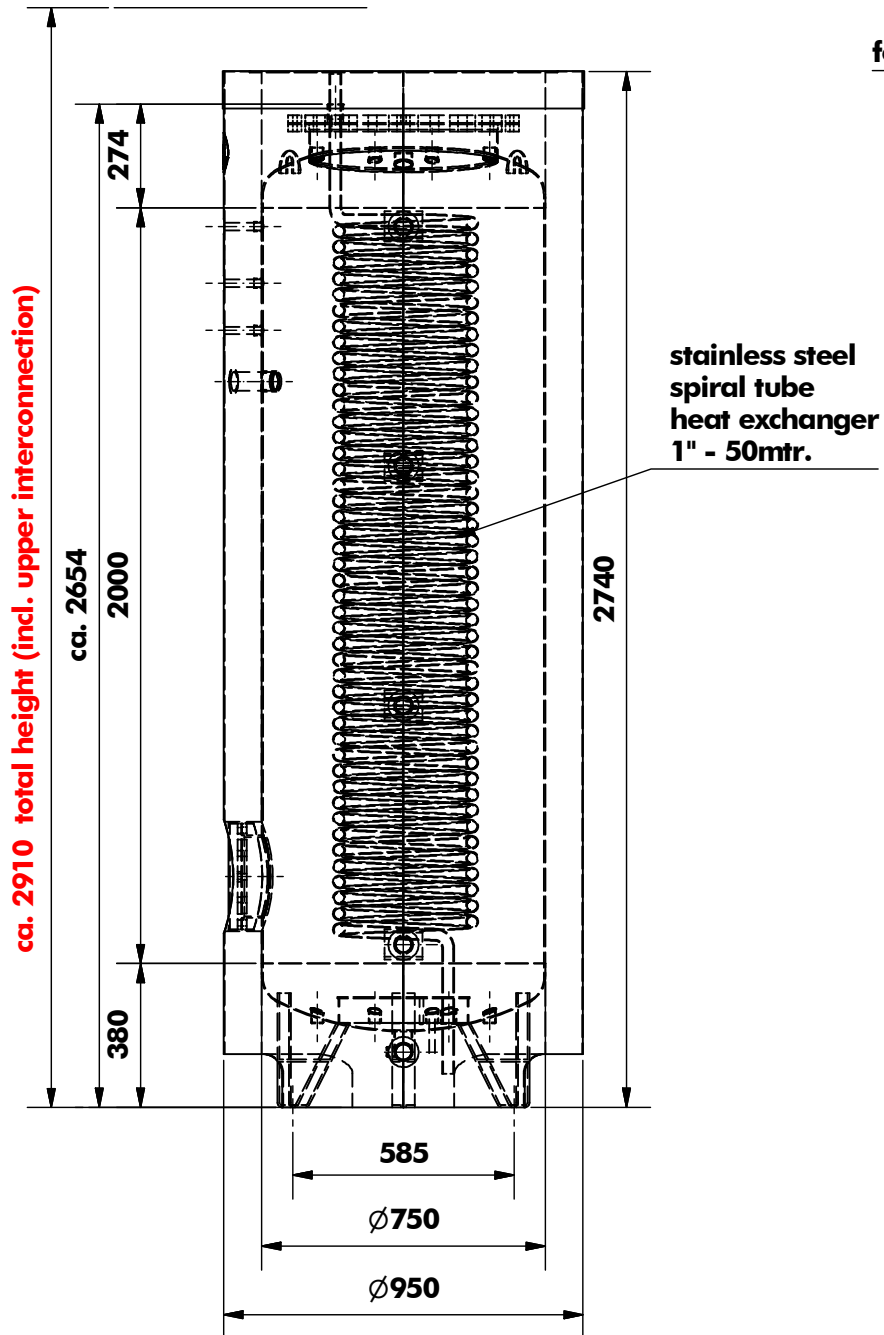
side view from the right side - without extendet heat exchangers -
