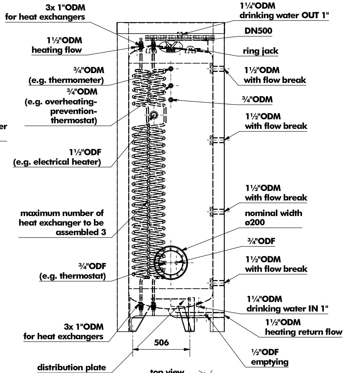
front view - without stainless steel spiral tube heat exchanger -
